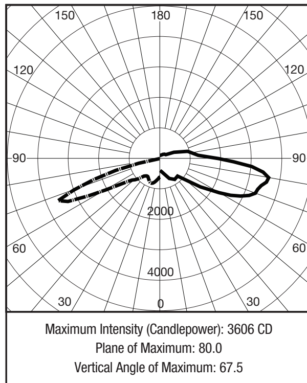
With Clear Curved Plastic Lenses over LEDs
