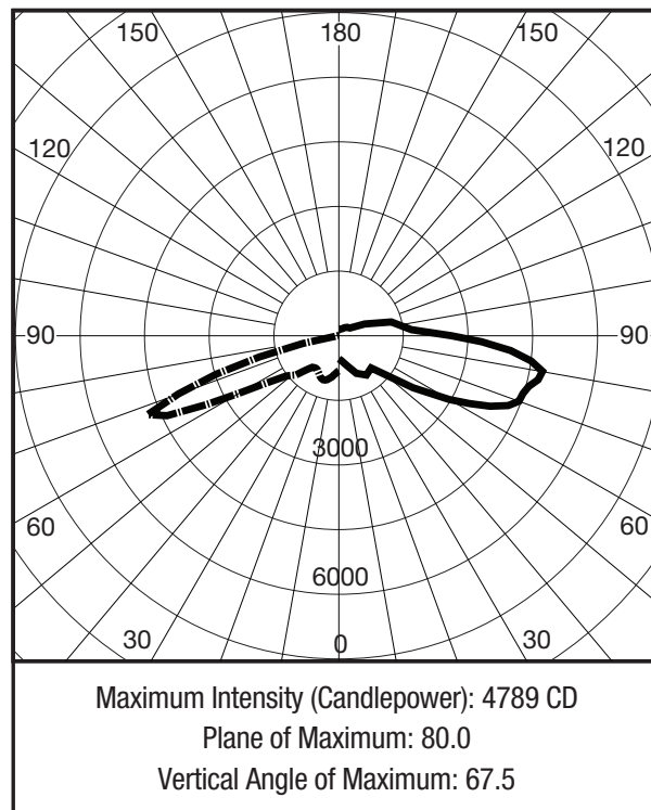
With Clear Curved Plastic Lenses over Leds
