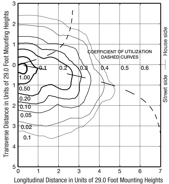
With Clear Curved Plastic Lenses over Leds
